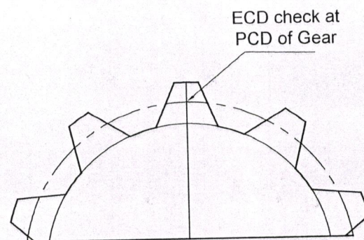
Gear Profile
